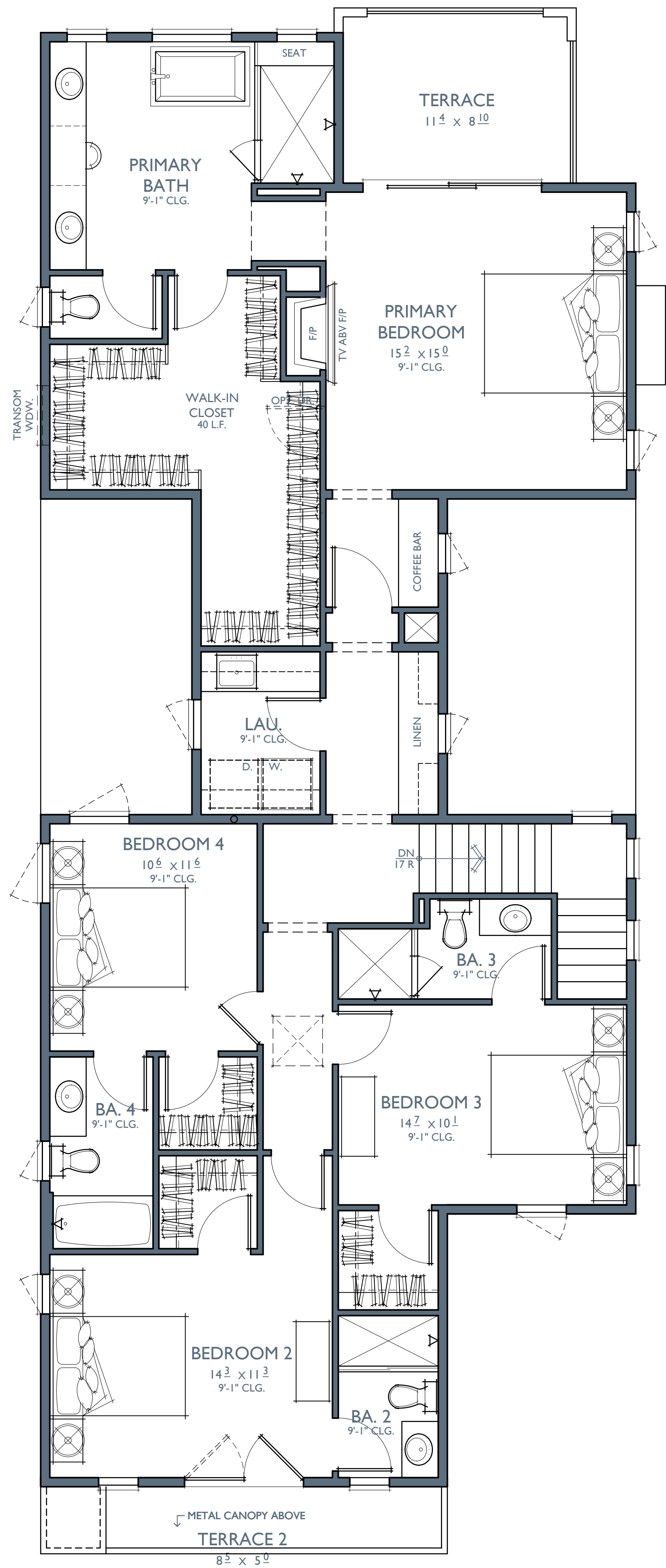
SECOND FLOOR
